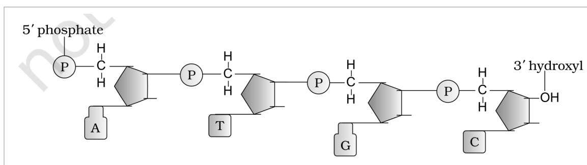
Figure 5.1 Polynucleotide chain. The 5' end carries a phosphate; the chain runs to the 3' end, which carries a free hydroxyl. Successive sugars are joined by 3'-5' phosphodiester linkages, and each sugar bears a nitrogenous base (the 5' Phosphate, Nitrogenous base, and 3' OH end are marked).
